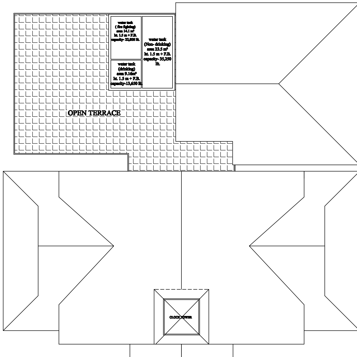
ROOF PLAN
