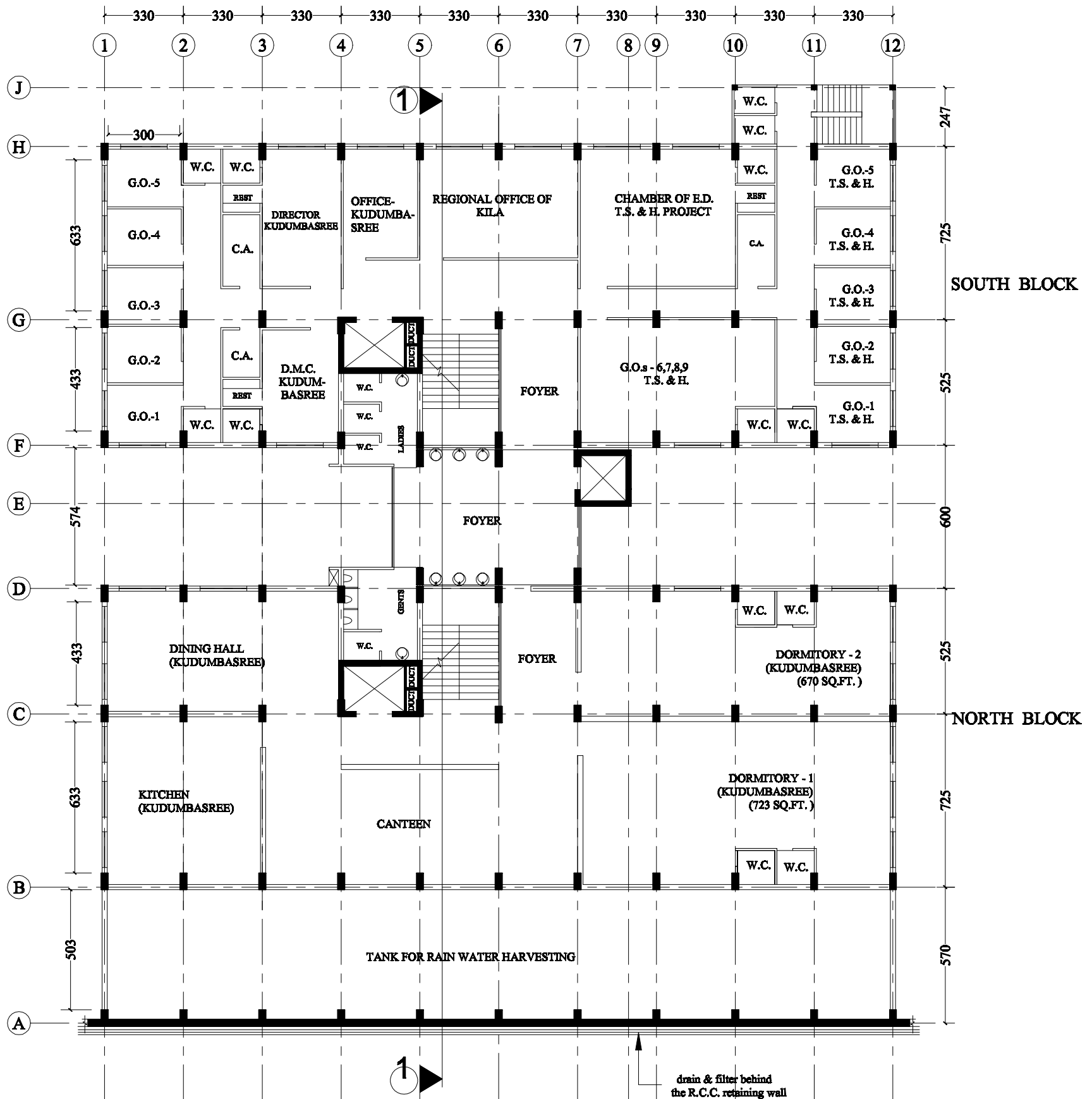
FLOOR -BASEMENT 1
